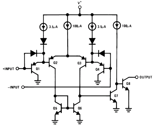
Logic Diagram
