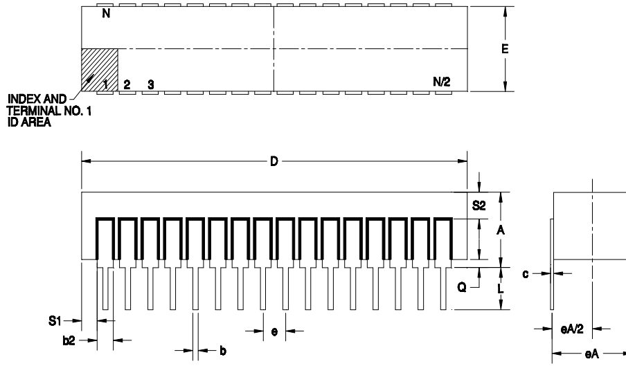
32 PIN DUAL IN-LINE PACKAGE 1,2
