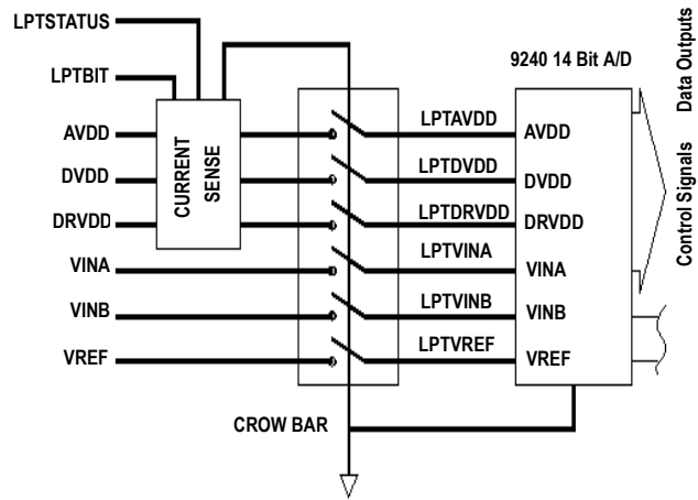
9240LP Block Diagram
