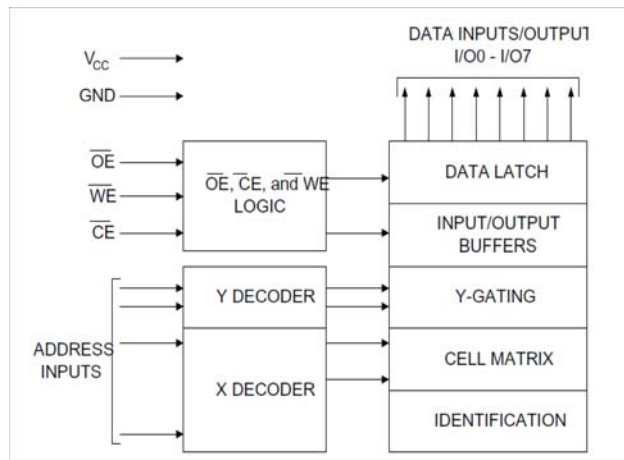
Logic Diagram
