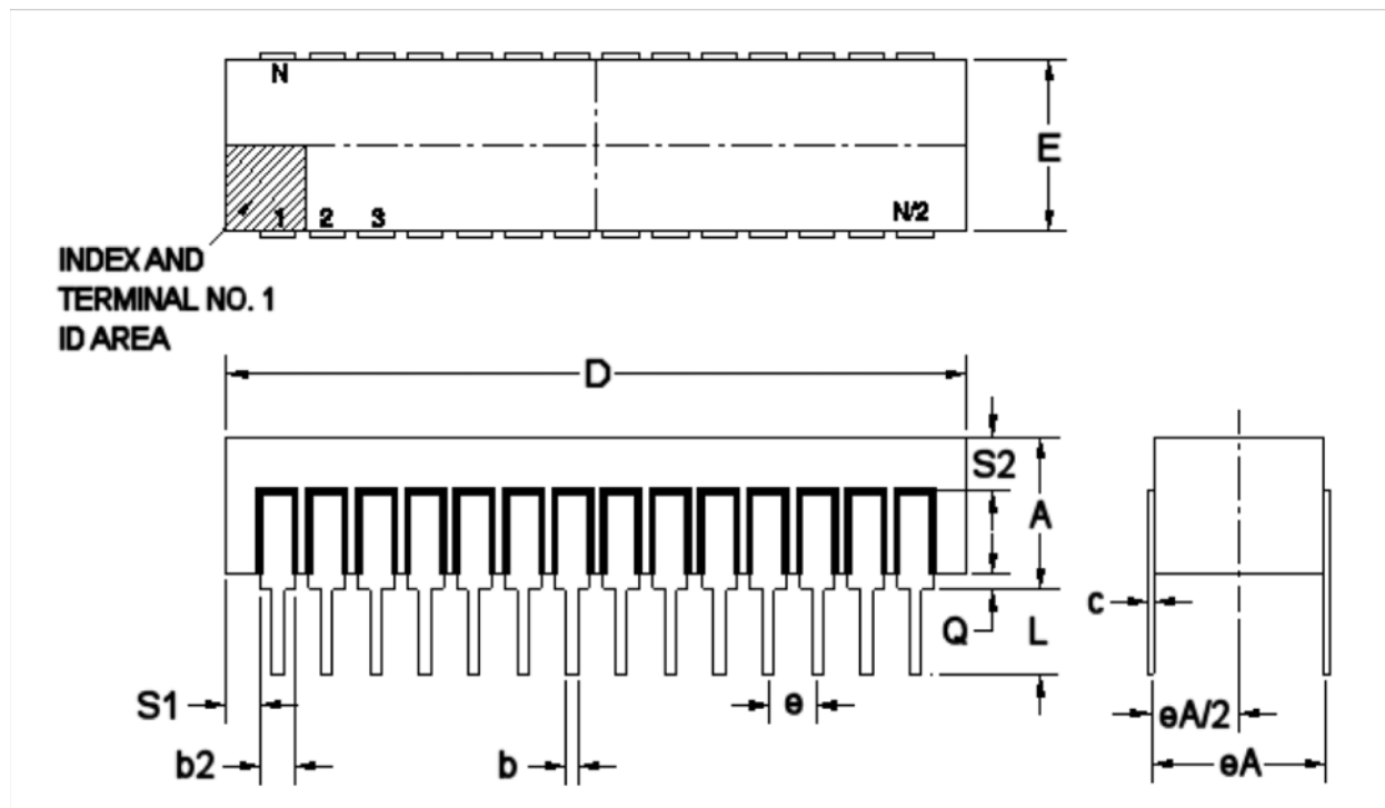
28 PIN RAD-PAK® DUAL IN LINE PACKAGE
