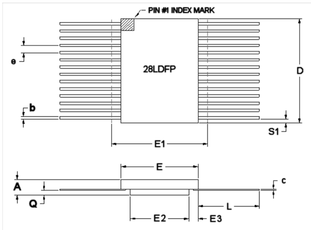
28 PIN RAD-PAK® FLAT PACKAGE
